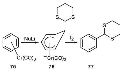
Scheme 22
