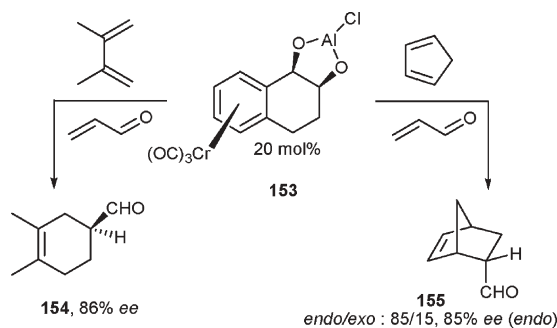
Scheme 43
