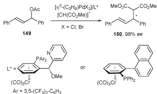
Scheme 41
