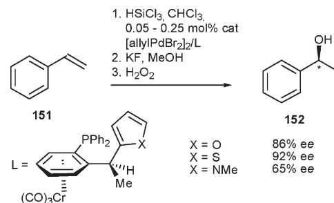
Scheme 42
